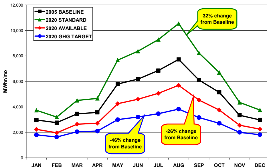
ENERGY DEMAND COMPARISON FOR 2005 BASELINE AND 2020 EFFICIENCY LEVELS
